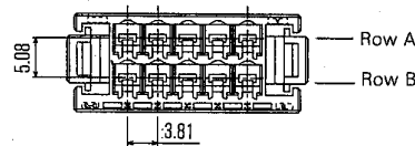
Horizontal/Vertical Type
